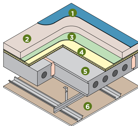
Robust Detail, E-FC-8
