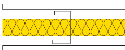
70mm Metal Stud Wall with 25mm APR 1200 & 12.5mm Plasterboard 42 dB ( R_w )
