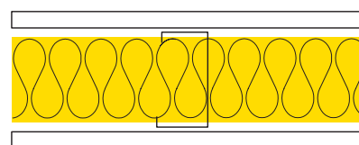
70mm Metal Stud Wall with 50mm APR 1200 & 12.5mm Plasterboard 43 dB ( R_w )
